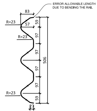
THRI-BEAM RAIL SECTION RAIL THICKNESS(2.67mm) CLASS A
