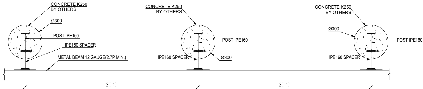
METAL BEAM GUARD RAIL WITH IPE160 STEEL POSTS BLOCKS PLAN
