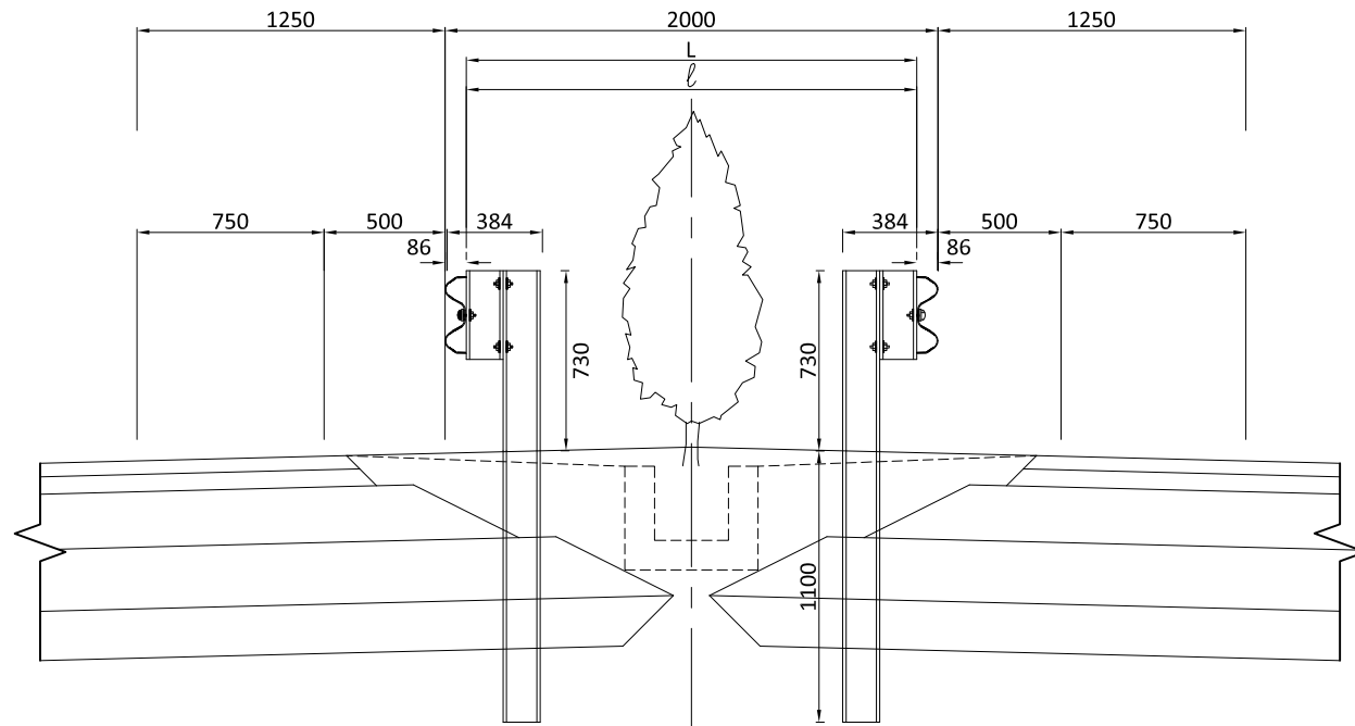
MEDIAN GUARD RAIL (INNER 4 LANE)
