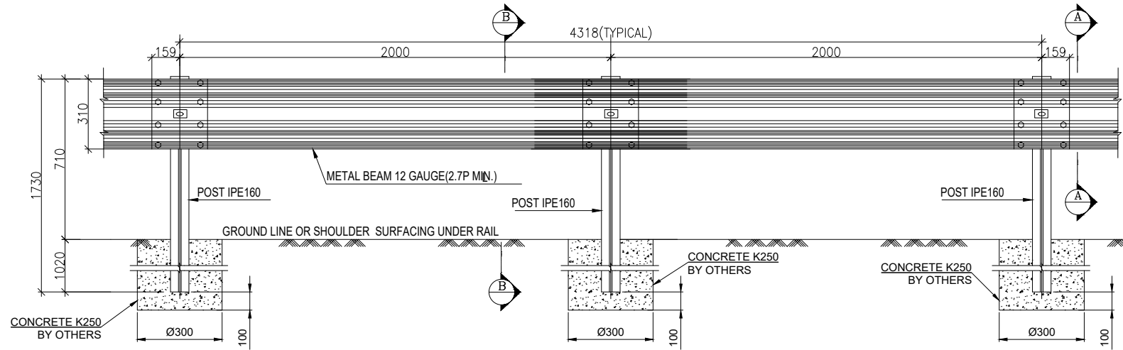
METAL BEAM GUARD RAIL WITH IPE 160 STEEL POSTS BLOCKS ELEVATION
